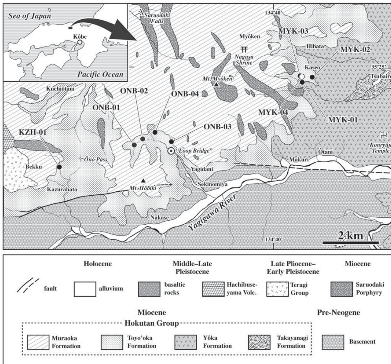
Fig. 1. Geologic map of study area with molluscan fossil localities. Geologic map after Editorial Committee of Engineering Geological Maps of Hyogo Prefecture ed. (1996).
